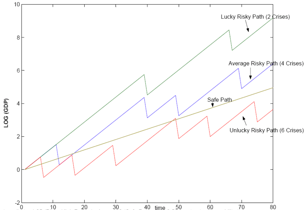
Figure 4: GDP Limit Distribution
